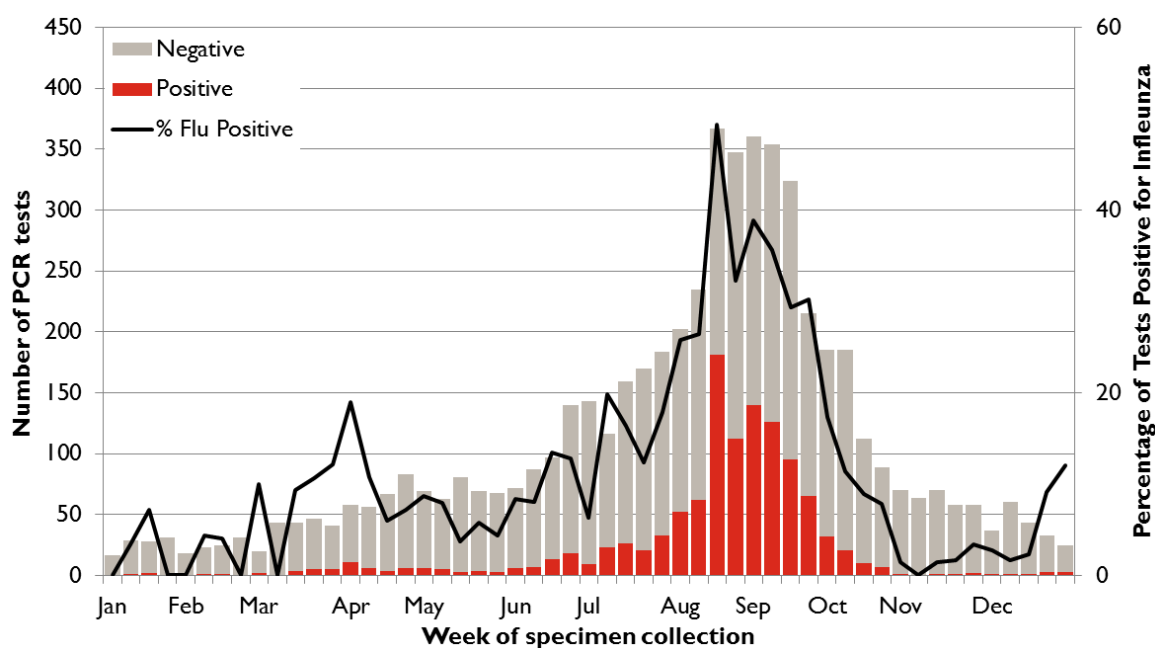
Figure 3: Influenza tests via PCR by week during 2015
